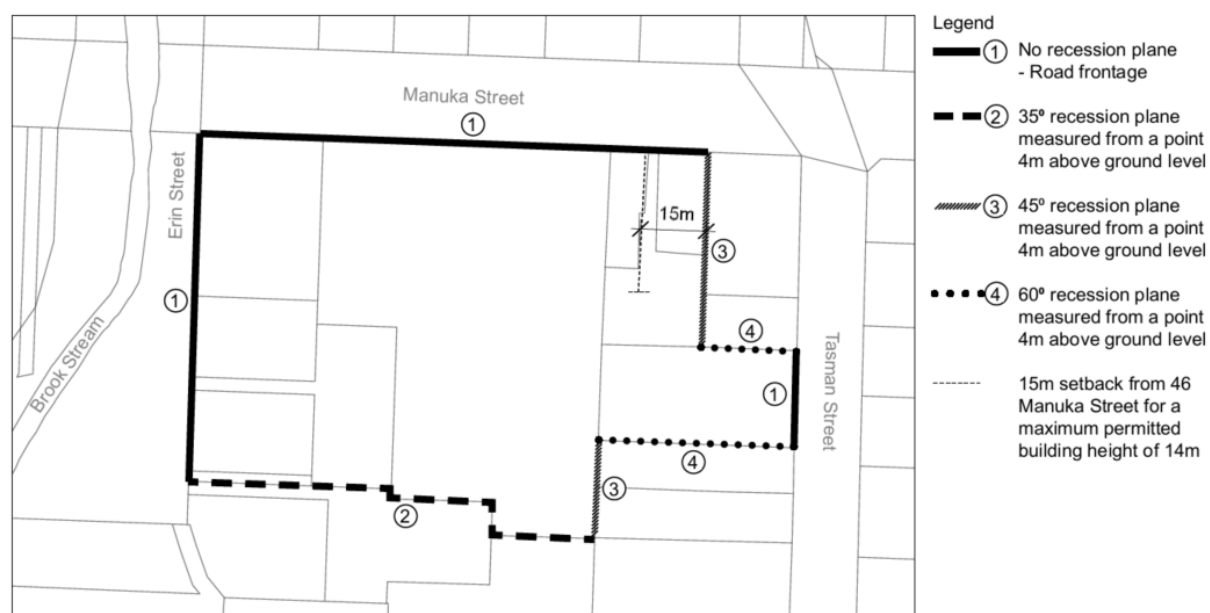
Figure 2 Diagram illustrating daylight admission standards contained in Table Y.3.7(h)
